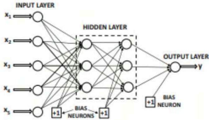
Gambar 2.3: Arsitektur feed-forward neural network (Aggarwal, 2018)
